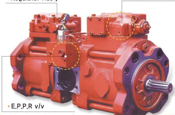
• Regulator Ass'y
